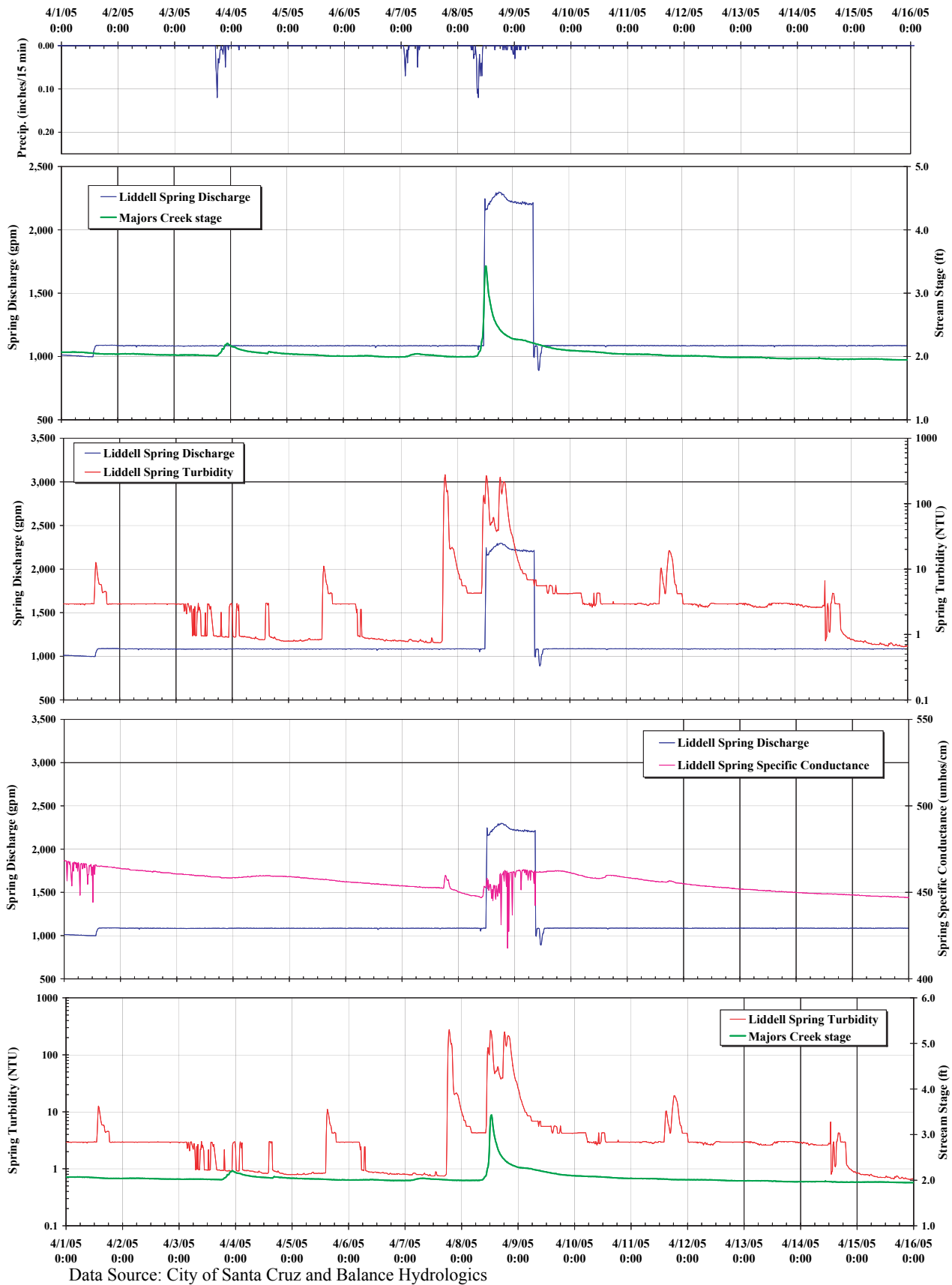
Storm Hydrograph Comparison, April 2005
